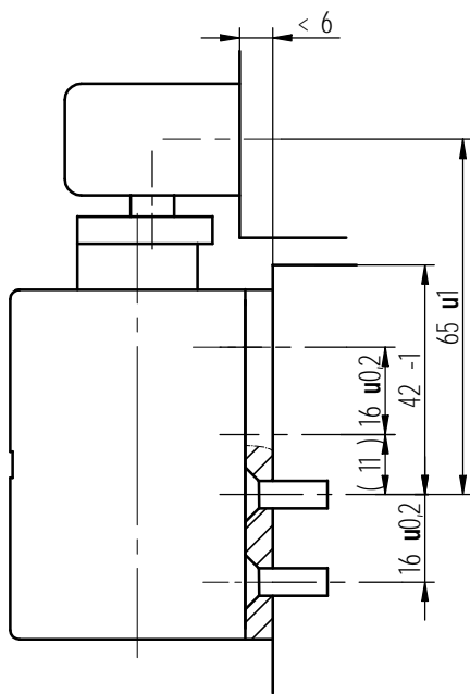
DIN links left hand door
